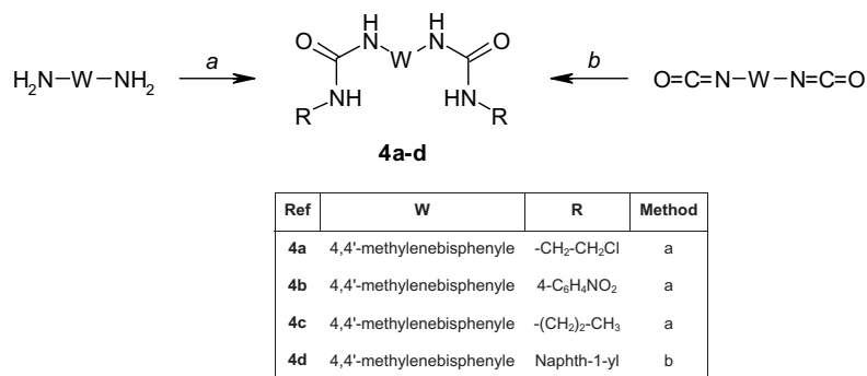
Scheme 4. Reagents and conditions: (a) R–NCO/diethyl ether/rt; (b) Ar–NH 2 /diethyl ether/rt.
