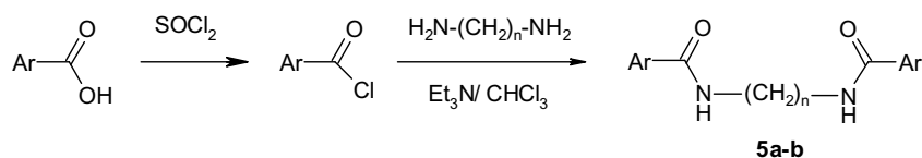
Scheme 5. 5a : Ar: pyrid-3-yl; n = 12; 5b : Ar: quinol-3-yl; n = 3.
