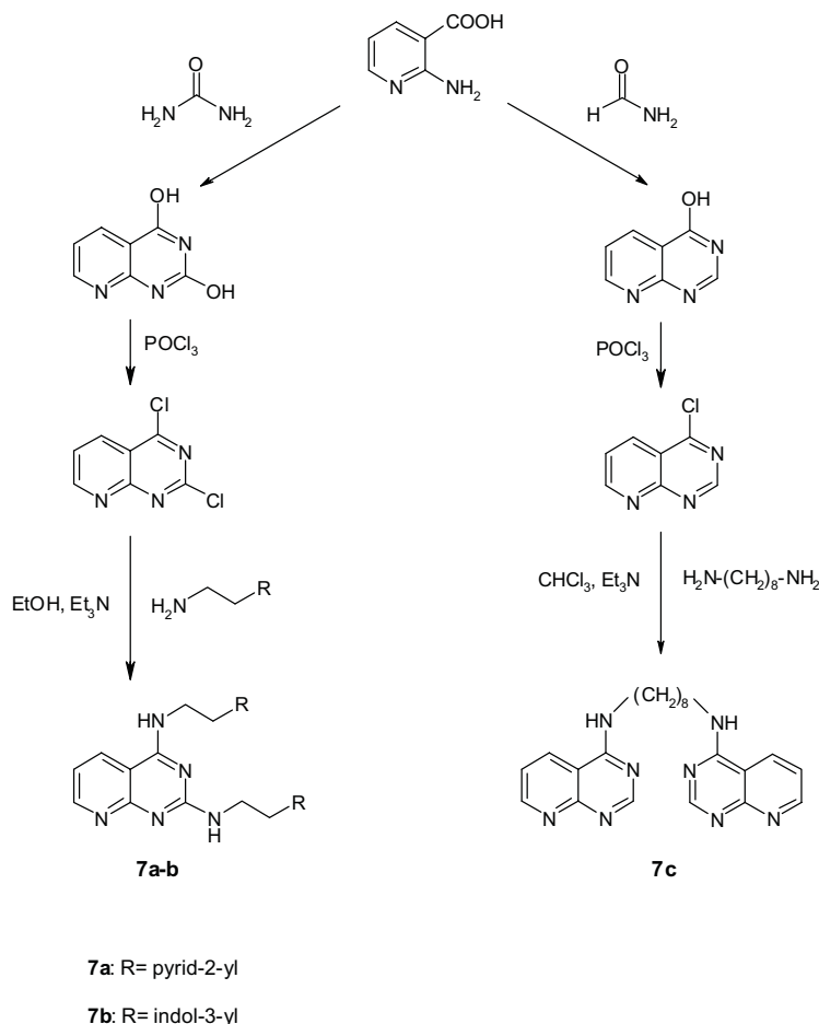
Scheme 6. 7a: R = pyrid-2-yl; 7b: R = indol-3-yl.
