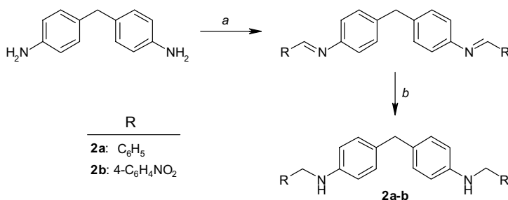
Scheme 2. Reagents and conditions: (a) R-CHO/diethyl ether/molecular sieves (4 Å)/rt; (b) methanol:HCl(c) (8:2, v:v)/NaCBH 3 /rt.
